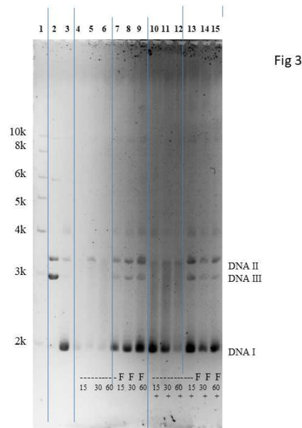
Figure 3: Denaturing and Renaturing Super Coiled pBluescript DNA (AGE in 1% agarose) Carried out in TBE Buffer with 1 \mu g Chloroquine/ml at RT with 2v/cm.)
