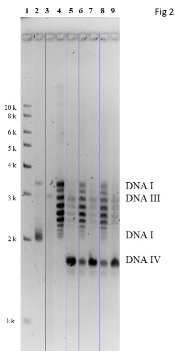
Figure 2: Denaturing and Renaturing Relaxed pBluscript DNA (AGE in 1% Agaroseis Carried Out in TBE Buffer with 1 \mu g Chloroquine/ml at RT with 5v/cm.)
