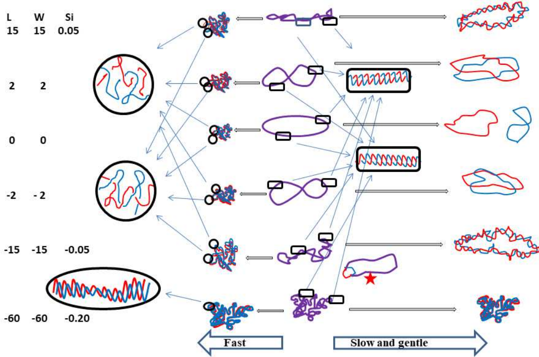
Figure 4: Schematic Possible Shapes of Differently Super Coiled Plasmid before and after Denaturing
