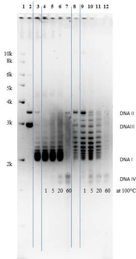
Figure 1: Super Coiled or Relaxed pBluescript DNA heat Stability Test (AGE with 1% agarose in TBE Buffer is Carried at RT with 2v/cm)
